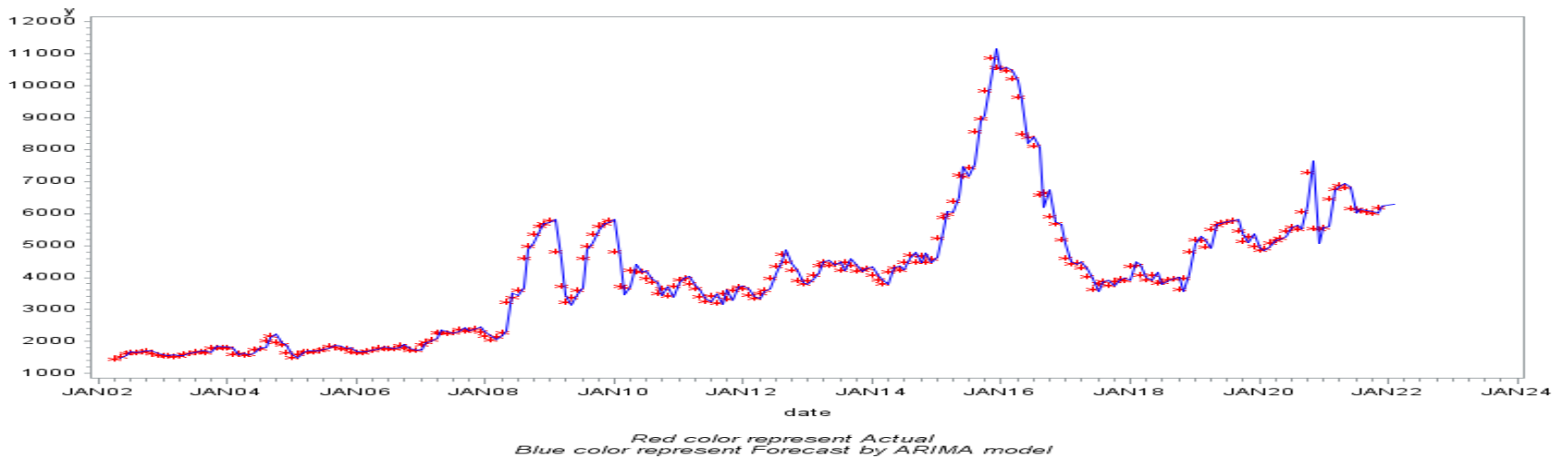
ARIMA fitting for Redgram price data
