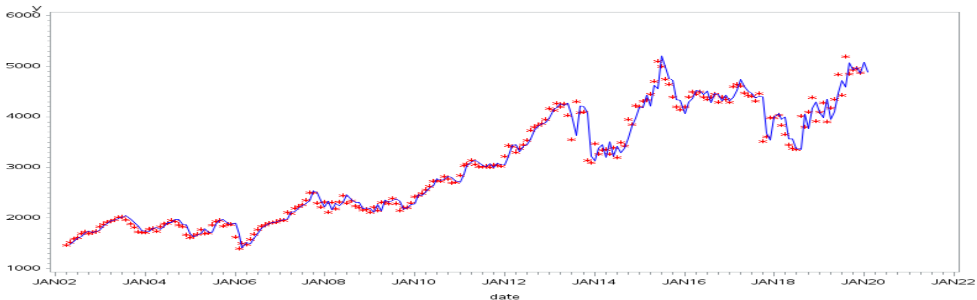
ARIMA fitting for Groundnut price data
