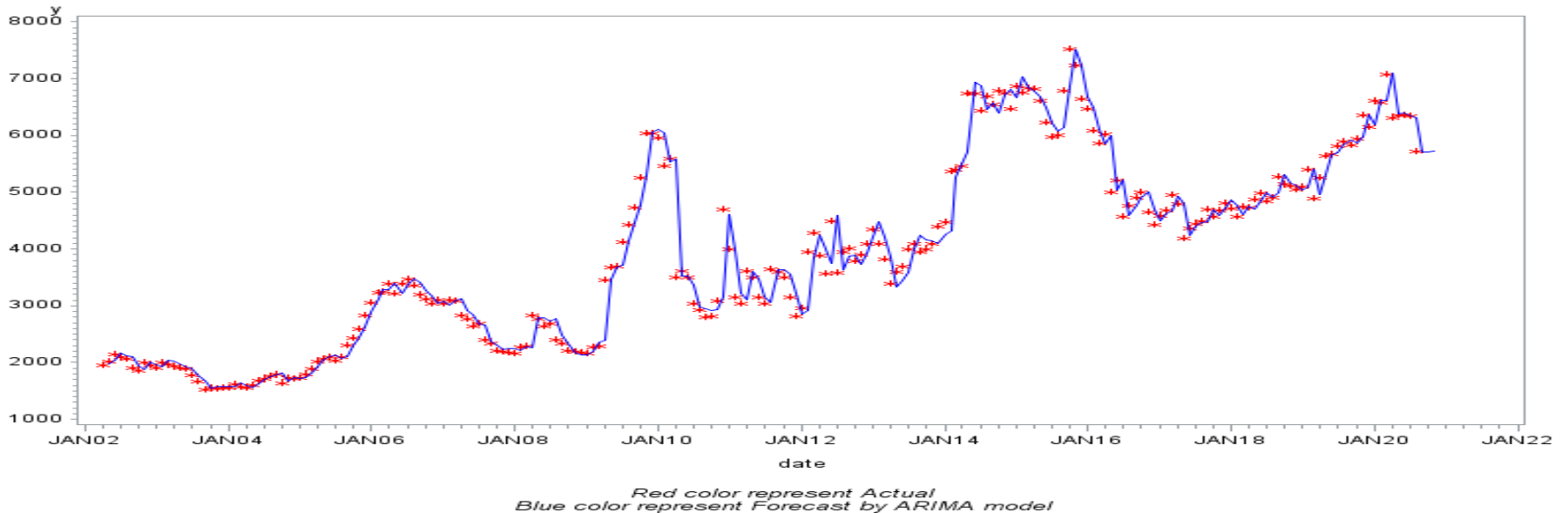
ARIMA fitting for Greengram price data
