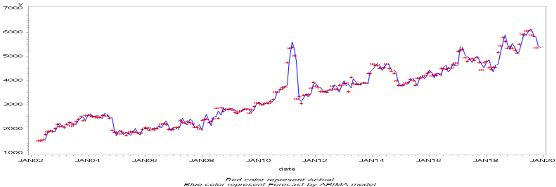
ARIMA fitting for cotton price data
