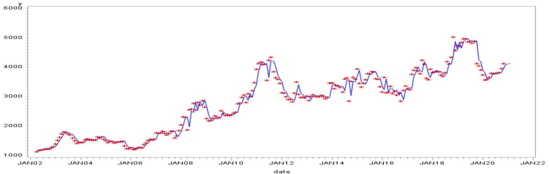
ARIMA fitting for Castor price data
